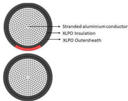
Figure 1 — Cross section: stranded aluminium conductor, XLPO insulation, XLPO outersheath. Red-striped and plain black variants.
